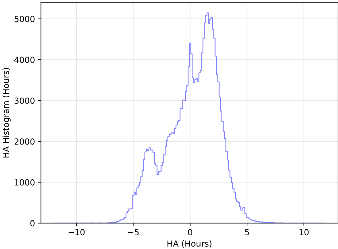
too_elab_r16_d3_ugrizy_v3.4_10yrs WFD g band: HA Histogram
