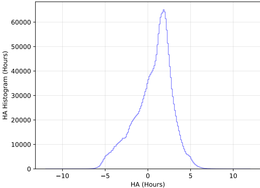
too_elab_r16_d3_ugrizy_v3.4_10yrs WFD all bands: HA Histogram
