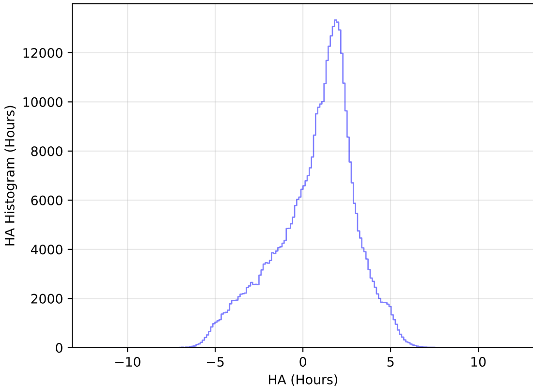
too_elab_r16_d3_ugrizy_v3.4_10yrs All sky z band: HA Histogram
