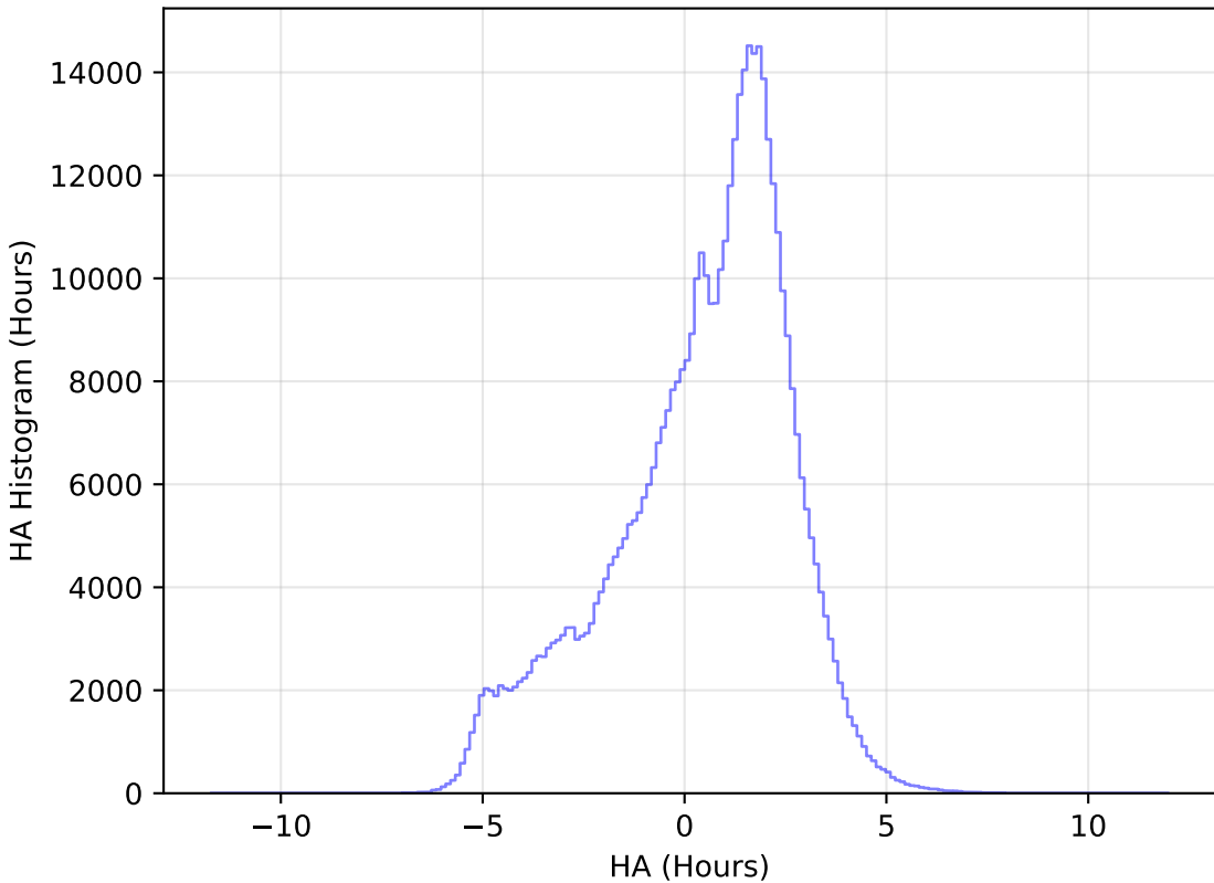
too_elab_r16_d3_ugrizy_v3.4_10yrs All sky r band: HA Histogram
