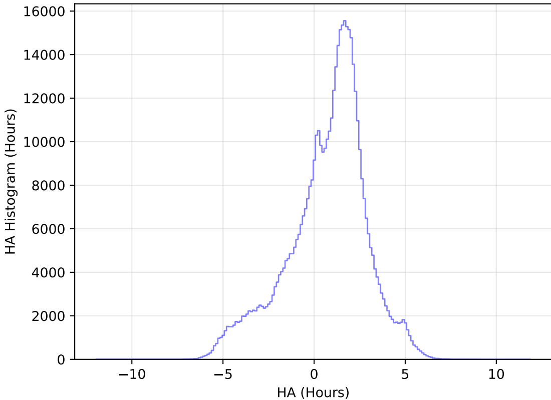
too_elab_r16_d3_ugrizy_v3.4_10yrs All sky i band: HA Histogram
