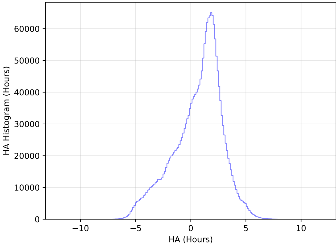
too_elab_r16_d3_ugrizy_v3.4_10yrs All sky all bands: HA Histogram
