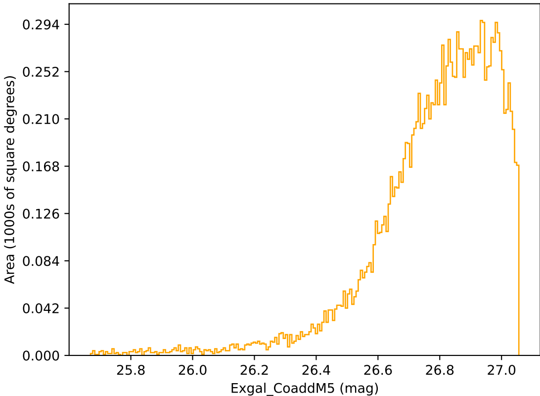
too_elab_r16_d3_ugrizy_v3.4_10yrs WFD r band: Exgal_CoaddM5
