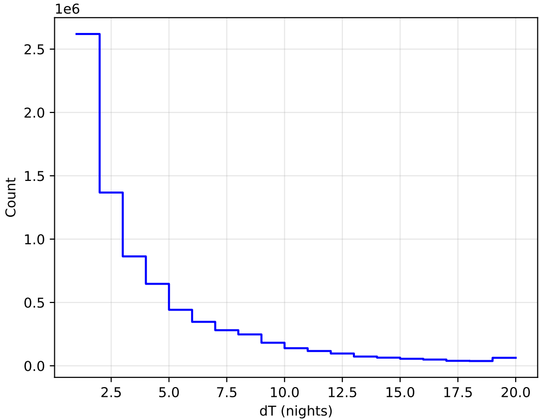
too_elab_r16_d3_ugrizy_v3.4_10yrs WFD all bands: DeltaNight Histogram
