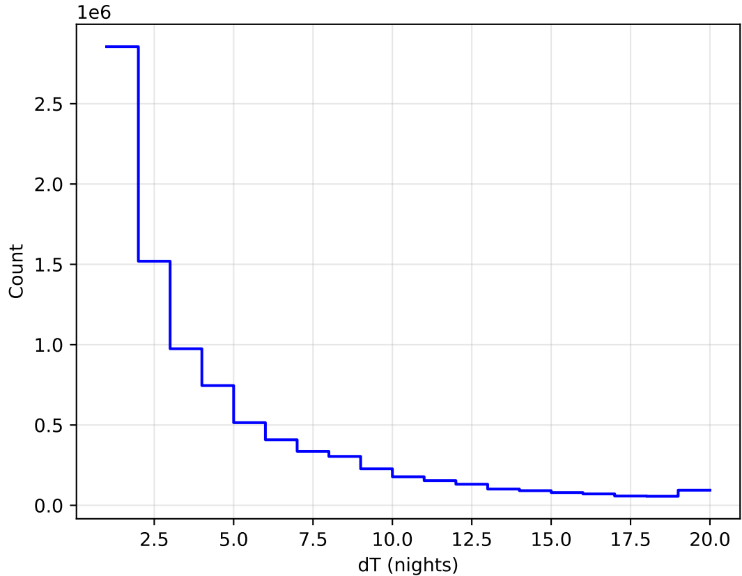
too_elab_r16_d3_ugrizy_v3.4_10yrs All sky all bands: DeltaNight Histogram
