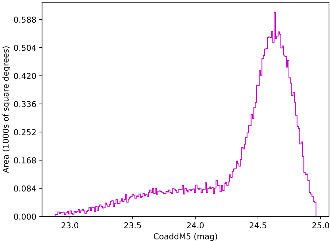
too_elab_r16_d3_ugrizy_v3.4_10yrs Yr 1 z band: CoaddM5
