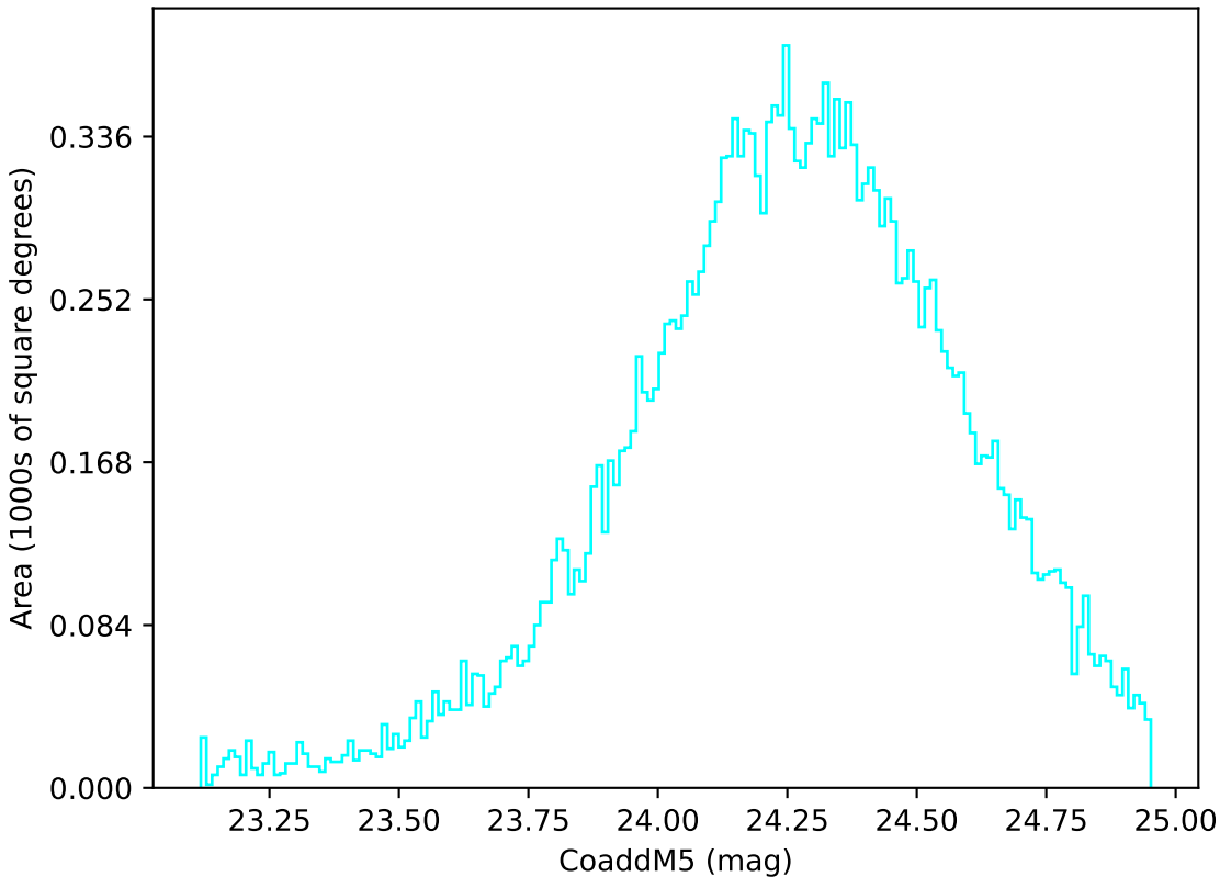
too_elab_r16_d3_ugrizy_v3.4_10yrs Yr 1 u band: CoaddM5
