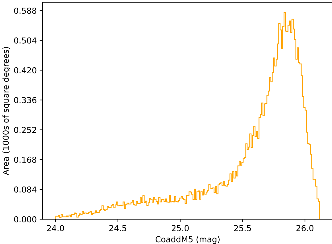
too_elab_r16_d3_ugrizy_v3.4_10yrs Yr 1 r band: CoaddM5
