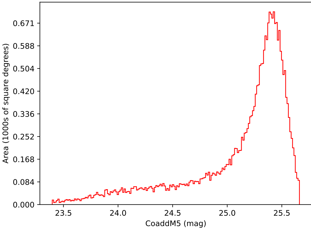
too_elab_r16_d3_ugrizy_v3.4_10yrs Yr 1 i band: CoaddM5
