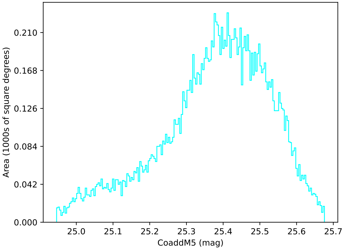
too_elab_r16_d3_ugrizy_v3.4_10yrs WFD u band: CoaddM5
