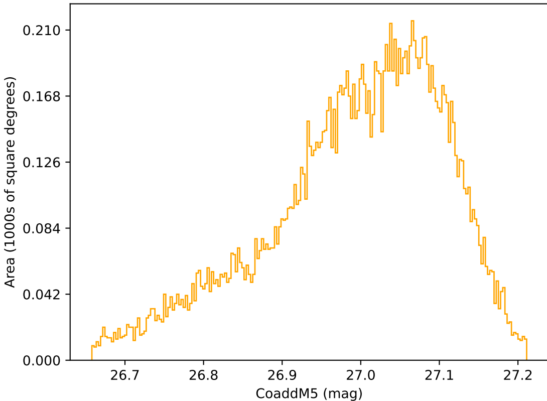
too_elab_r16_d3_ugrizy_v3.4_10yrs WFD r band: CoaddM5
