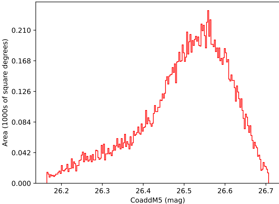
too_elab_r16_d3_ugrizy_v3.4_10yrs WFD i band: CoaddM5
