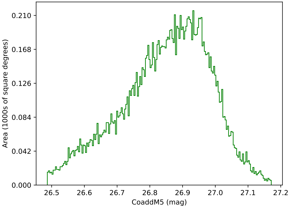
too_elab_r16_d3_ugrizy_v3.4_10yrs WFD g band: CoaddM5
