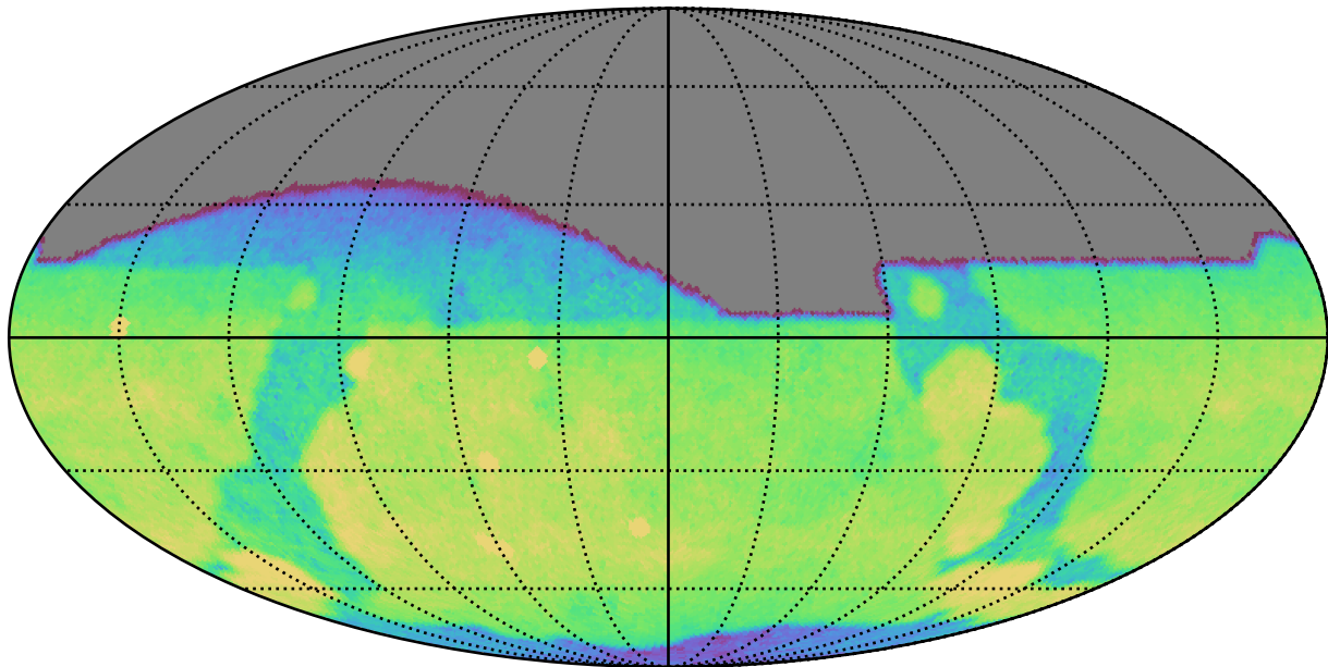
too_elab_r16_d3_ugrizy_v3.4_10yrs All sky g band: CoaddM5
