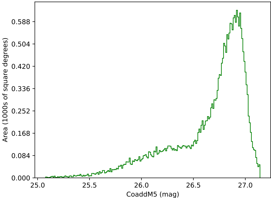
too_elab_r16_d3_ugrizy_v3.4_10yrs All sky g band: CoaddM5
