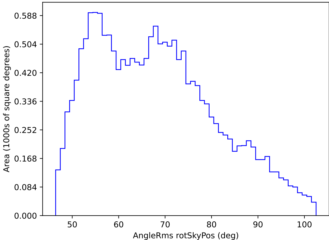
too_elab_r16_d3_ugrizy_v3.4_10yrs WFD g band: AngleRms rotSkyPos
