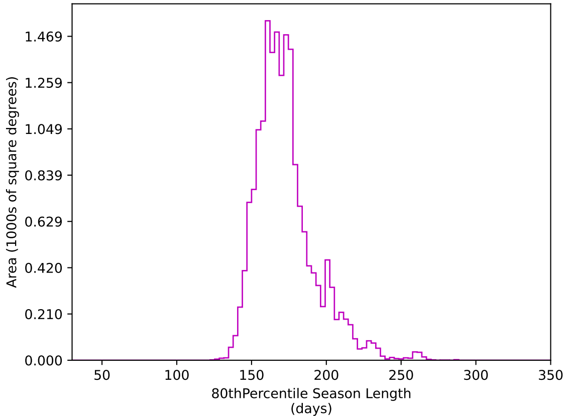
too_elab_r16_d3_ugrizy_v3.4_10yrs WFD z band: 80thPercentile Season Length
