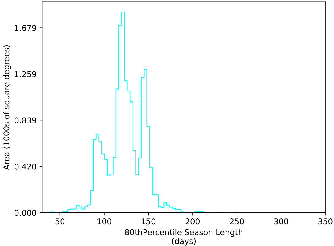
too_elab_r16_d3_ugrizy_v3.4_10yrs WFD u band: 80thPercentile Season Length
