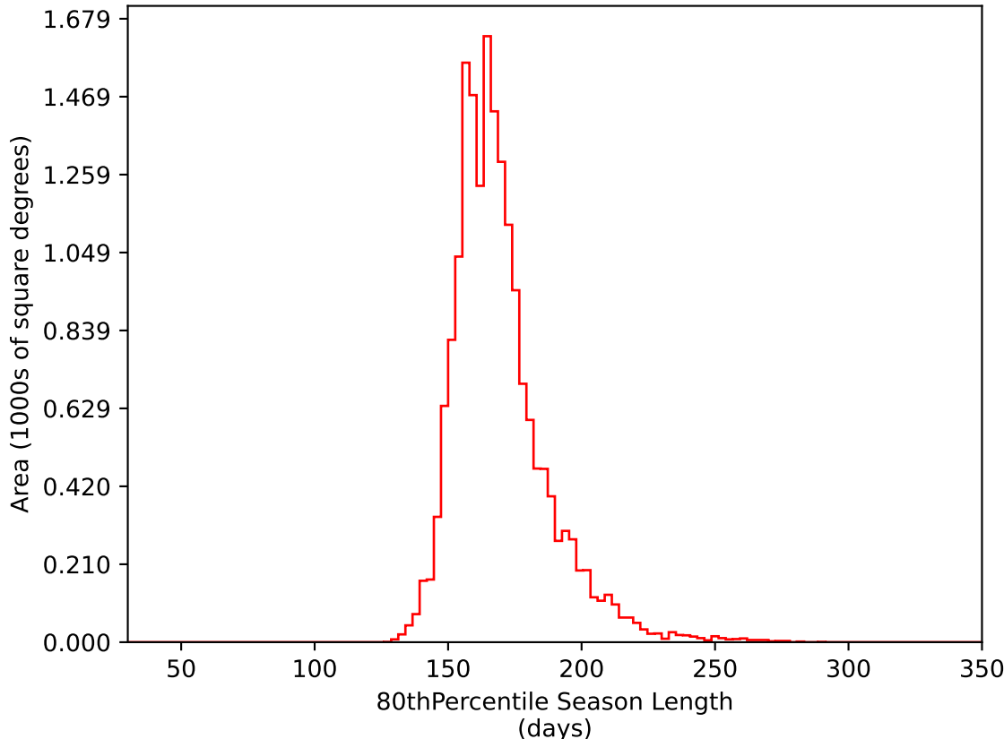
too_elab_r16_d3_ugrizy_v3.4_10yrs WFD i band: 80thPercentile Season Length
