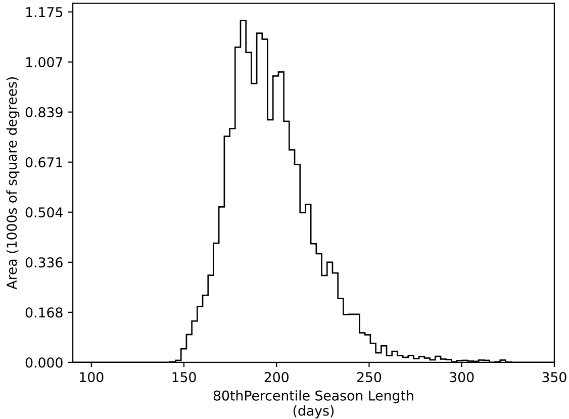
too_elab_r16_d3_ugrizy_v3.4_10yrs WFD all bands: 80thPercentile Season Length
