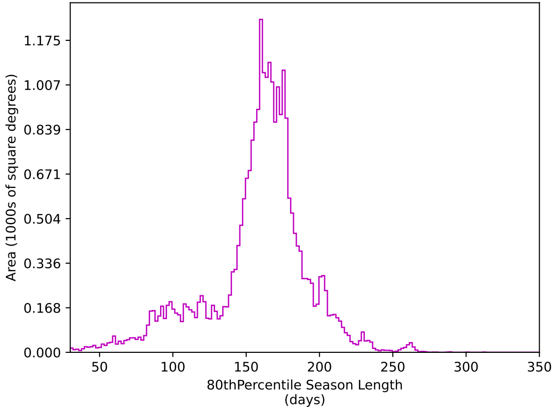
too_elab_r16_d3_ugrizy_v3.4_10yrs All sky z band: 80thPercentile Season Length
