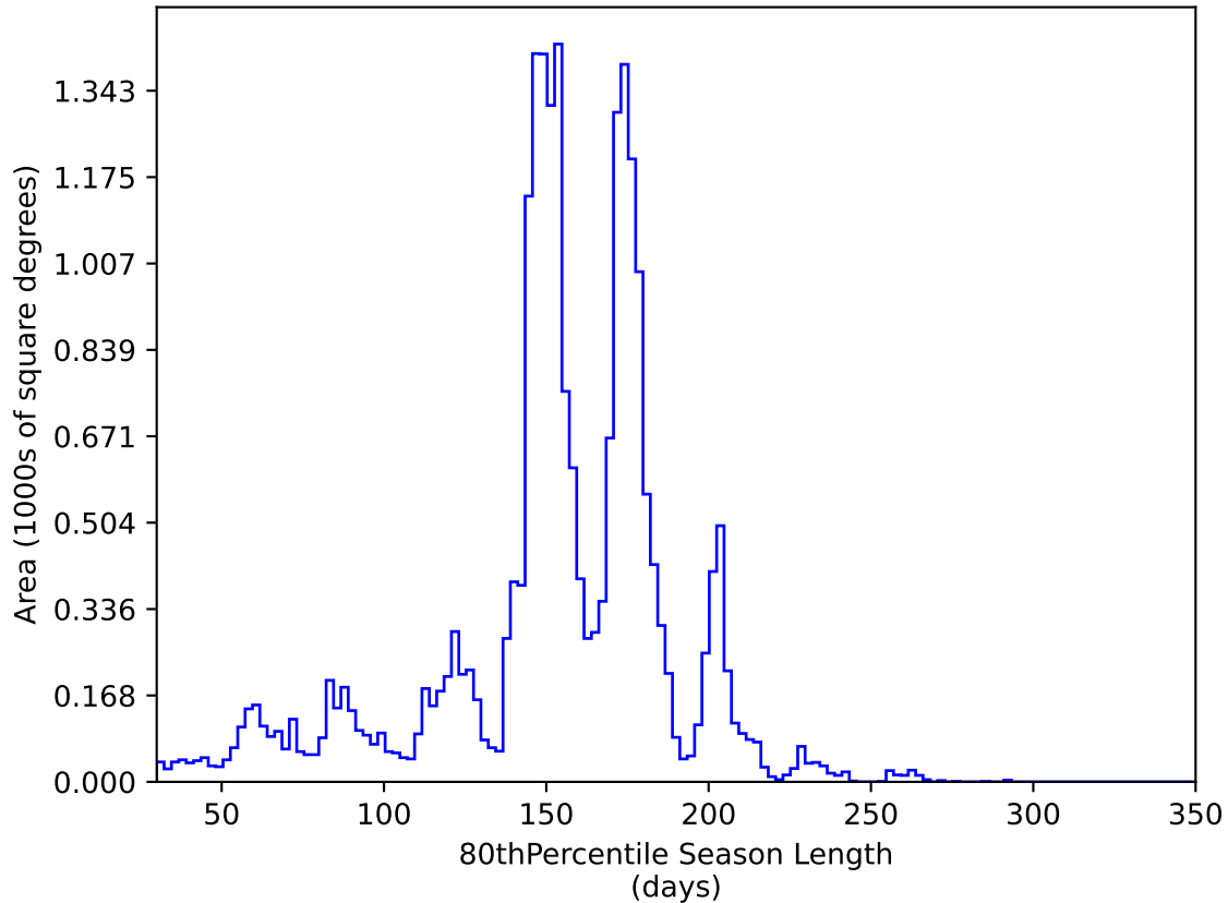
too_elab_r16_d3_ugrizy_v3.4_10yrs All sky y band: 80thPercentile Season Length
