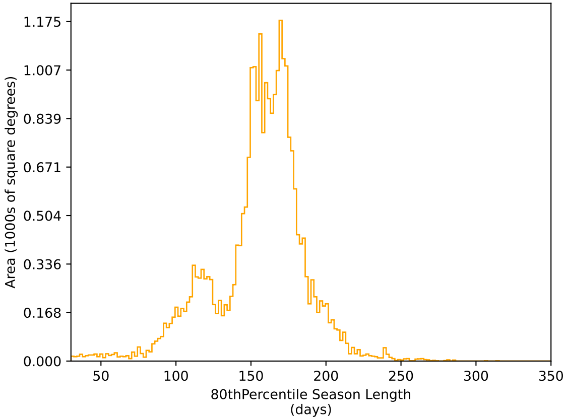
too_elab_r16_d3_ugrizy_v3.4_10yrs All sky r band: 80thPercentile Season Length
