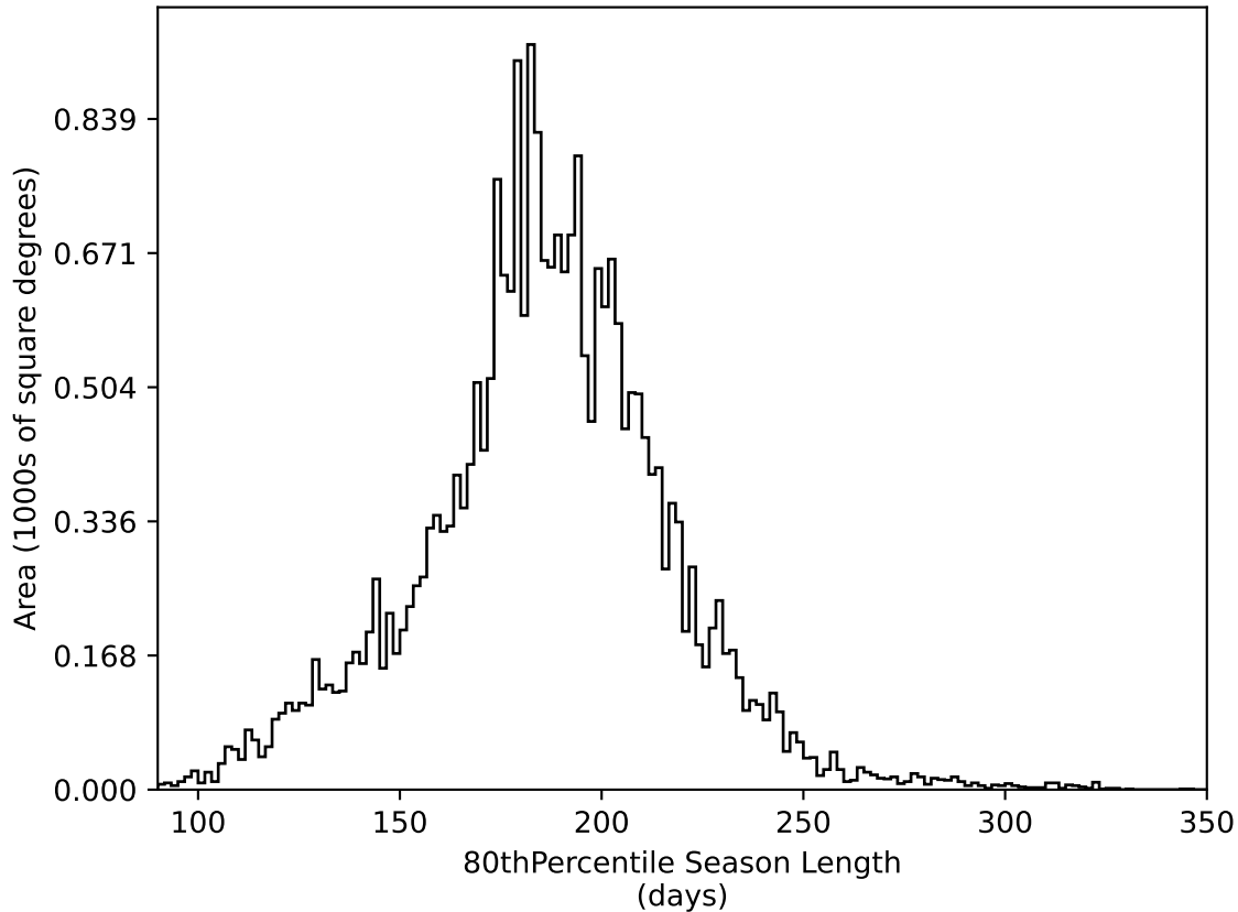
too_elab_r16_d3_ugrizy_v3.4_10yrs All sky all bands: 80thPercentile Season Length
