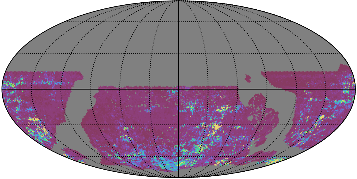
too_elab_r16_d3_ugrizy_v3.4_10yrs WFD z band: 75th Percentile Intranight Timespan
