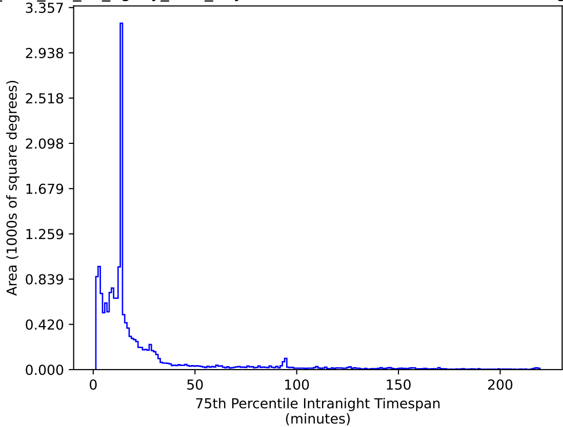
too_elab_r16_d3_ugrizy_v3.4_10yrs WFD z band: 75th Percentile Intranight Timespan
