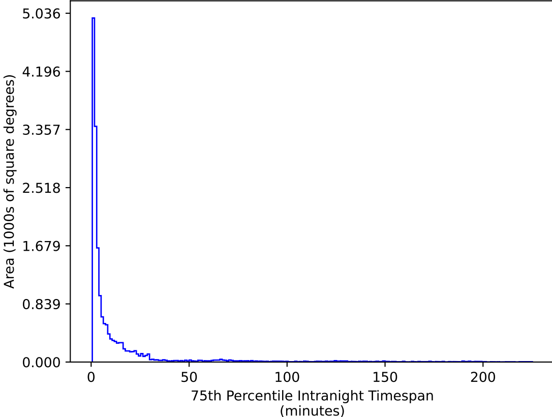
too_elab_r16_d3_ugrizy_v3.4_10yrs WFD u band: 75th Percentile Intranight Timespan
