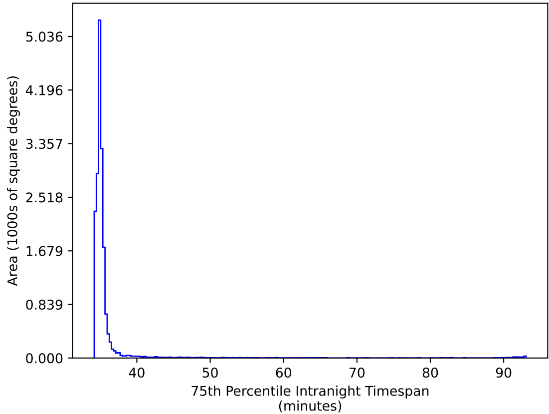
too_elab_r16_d3_ugrizy_v3.4_10yrs WFD ri bands: 75th Percentile Intranight Timespan
