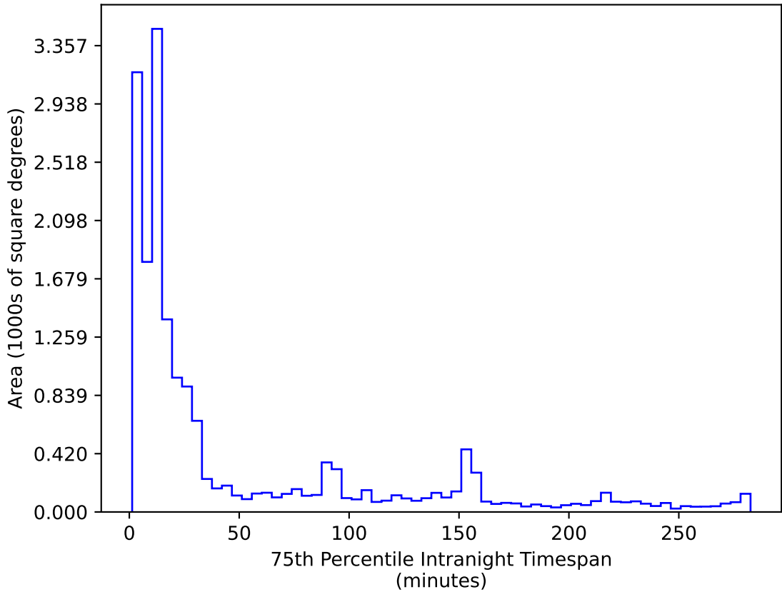
too_elab_r16_d3_ugrizy_v3.4_10yrs WFD r band: 75th Percentile Intranight Timespan
