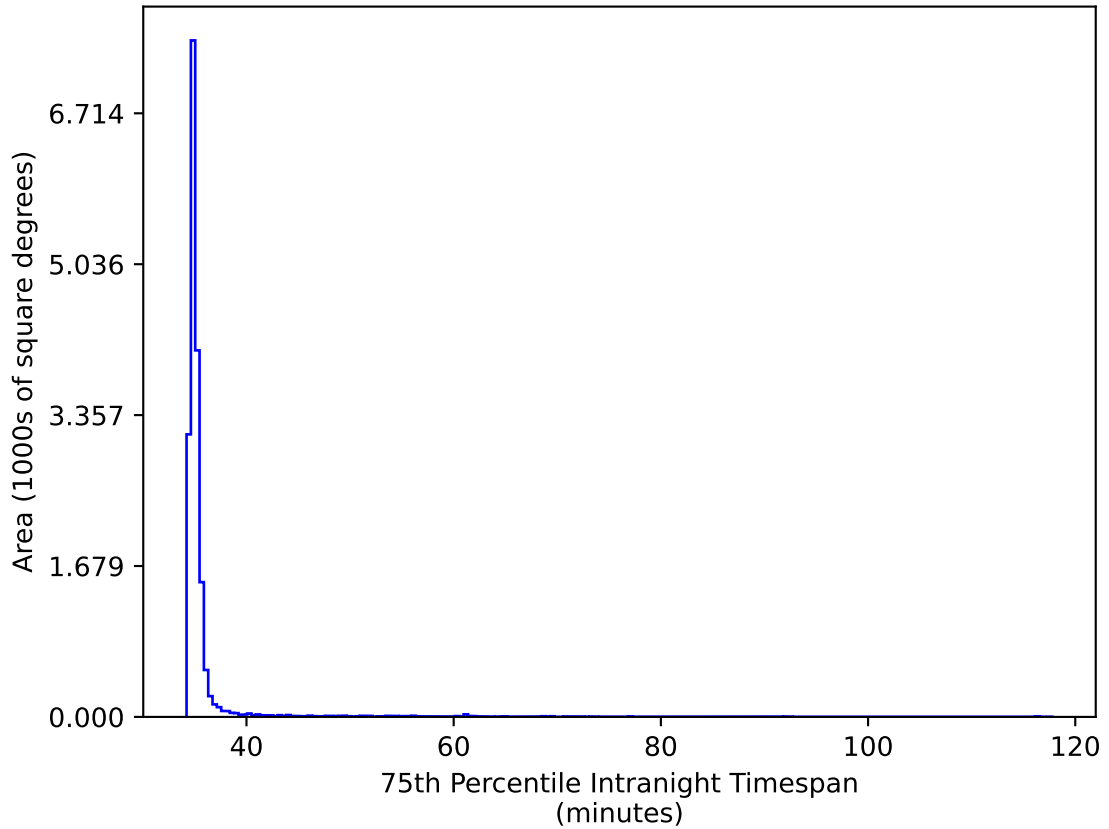
too_elab_r16_d3_ugrizy_v3.4_10yrs WFD gr bands: 75th Percentile Intranight Timespan
