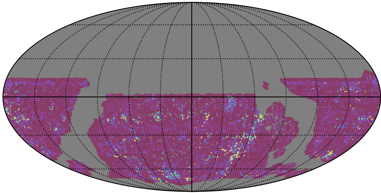
too_elab_r16_d3_ugrizy_v3.4_10yrs WFD g band: 75th Percentile Intranight Timespan
