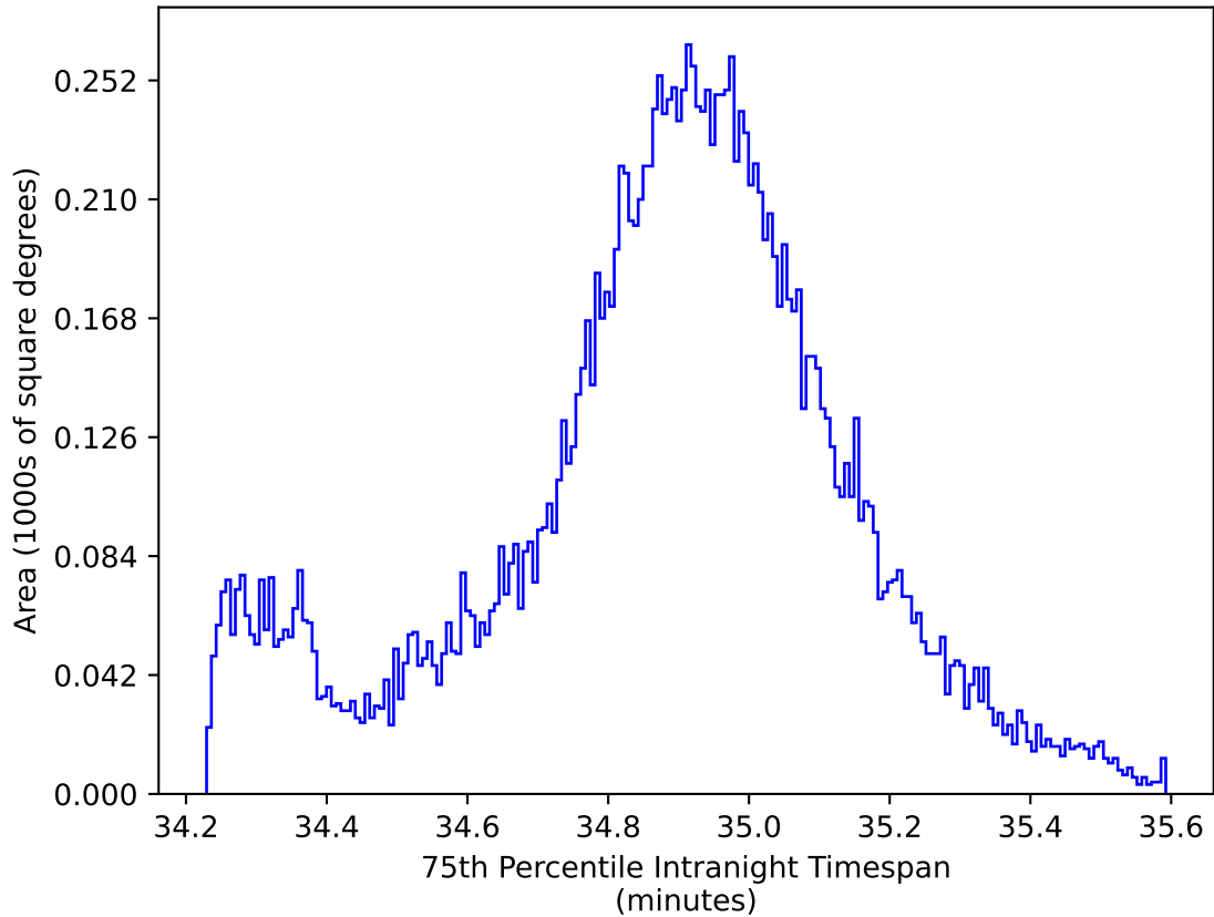
too_elab_r16_d3_ugrizy_v3.4_10yrs WFD all bands: 75th Percentile Intranight Timespan
