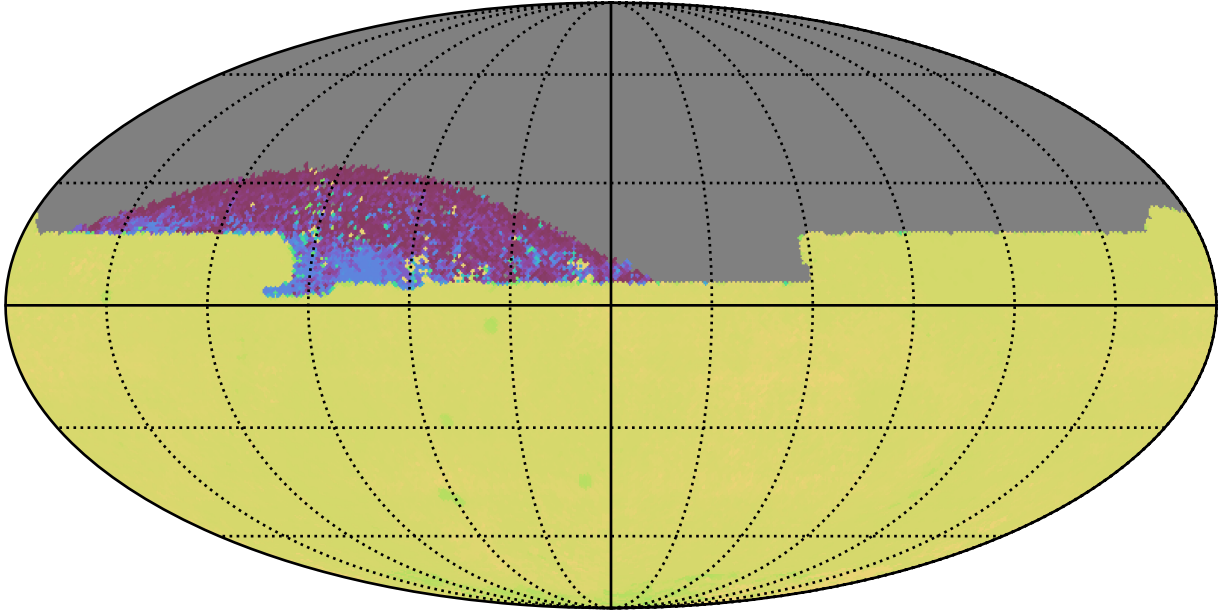
too_elab_r16_d3_ugrizy_v3.4_10yrs All sky zy bands: 75th Percentile Intranight Timespan
