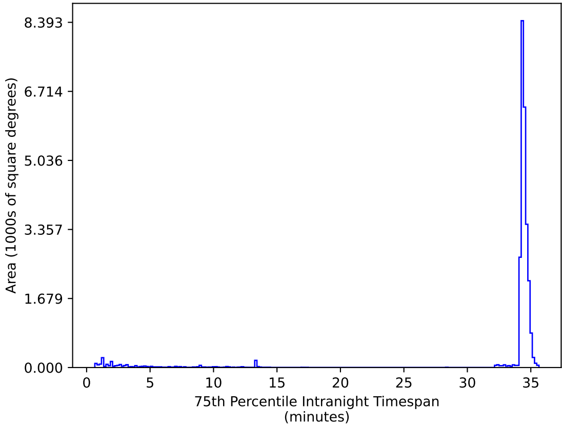
too_elab_r16_d3_ugrizy_v3.4_10yrs All sky zy bands: 75th Percentile Intranight Timespan
