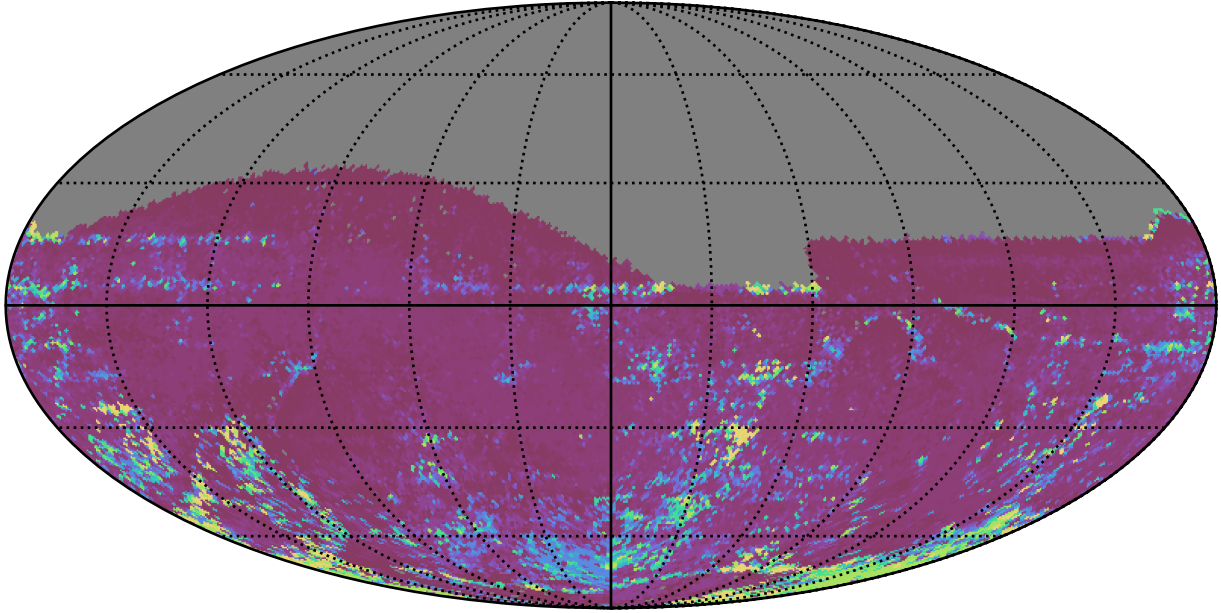
too_elab_r16_d3_ugrizy_v3.4_10yrs All sky z band: 75th Percentile Intranight Timespan
