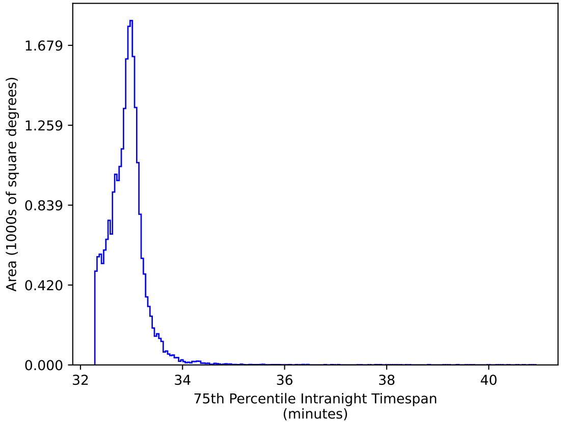
too_elab_r16_d3_ugrizy_v3.4_10yrs All sky y band: 75th Percentile Intranight Timespan
