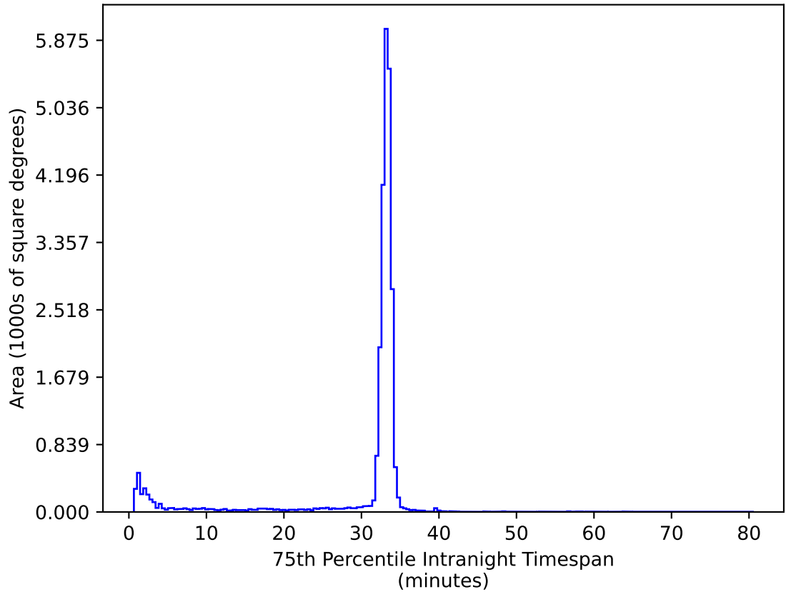
too_elab_r16_d3_ugrizy_v3.4_10yrs All sky ug bands: 75th Percentile Intranight Timespan
