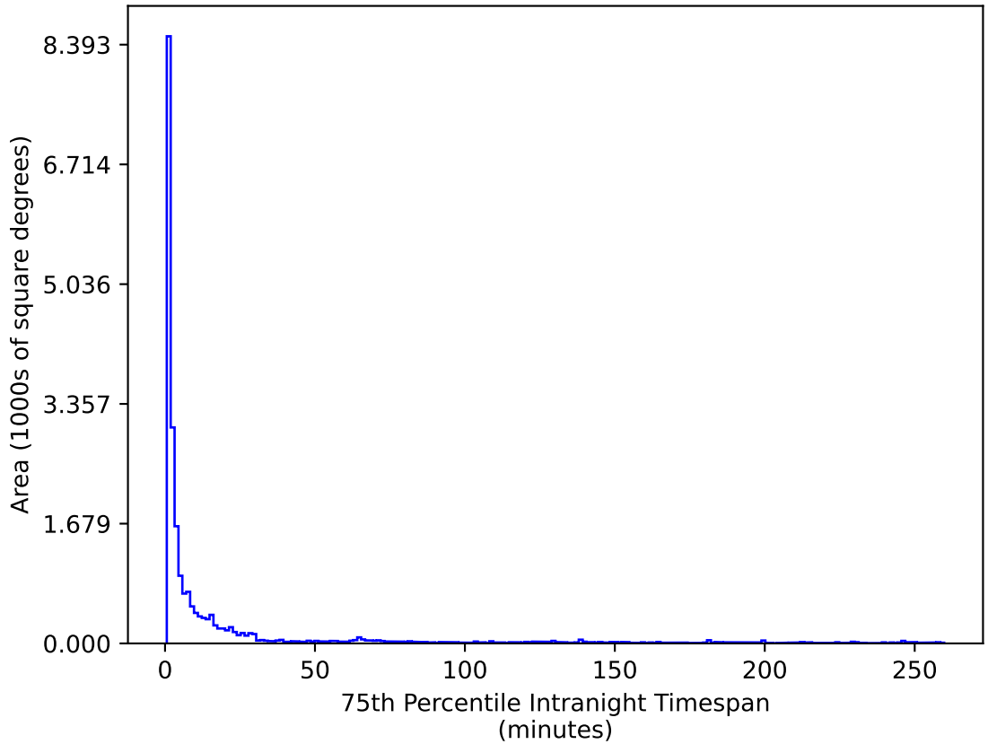
too_elab_r16_d3_ugrizy_v3.4_10yrs All sky u band: 75th Percentile Intranight Timespan
