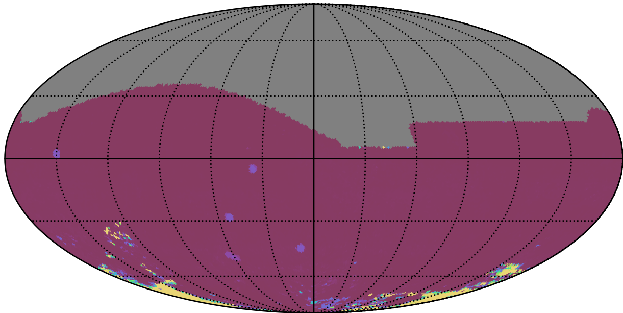
too_elab_r16_d3_ugrizy_v3.4_10yrs All sky iz bands: 75th Percentile Intranight Timespan
