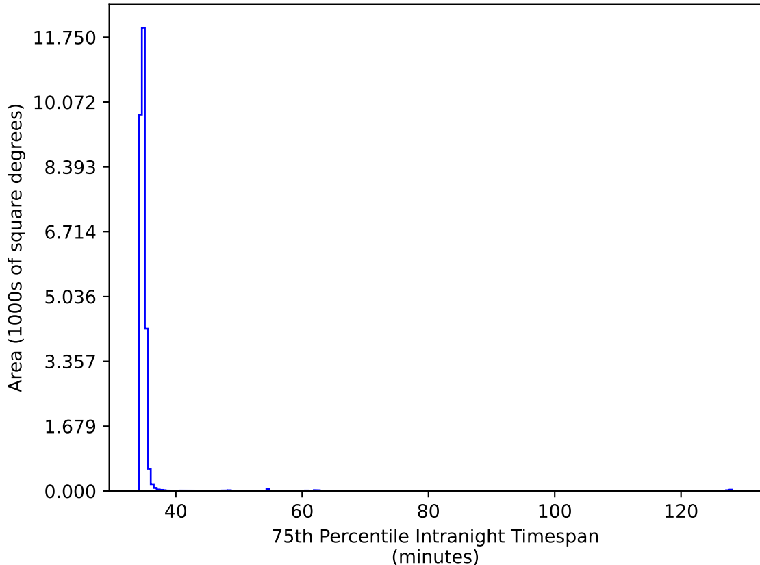
too_elab_r16_d3_ugrizy_v3.4_10yrs All sky iz bands: 75th Percentile Intranight Timespan
