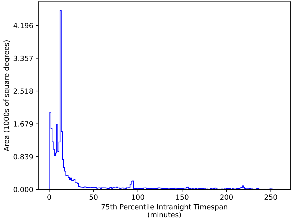
too_elab_r16_d3_ugrizy_v3.4_10yrs All sky i band: 75th Percentile Intranight Timespan
