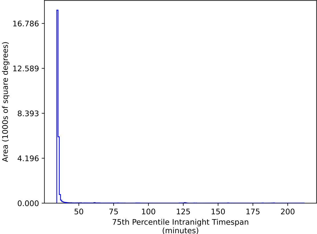
too_elab_r16_d3_ugrizy_v3.4_10yrs All sky gr bands: 75th Percentile Intranight Timespan
