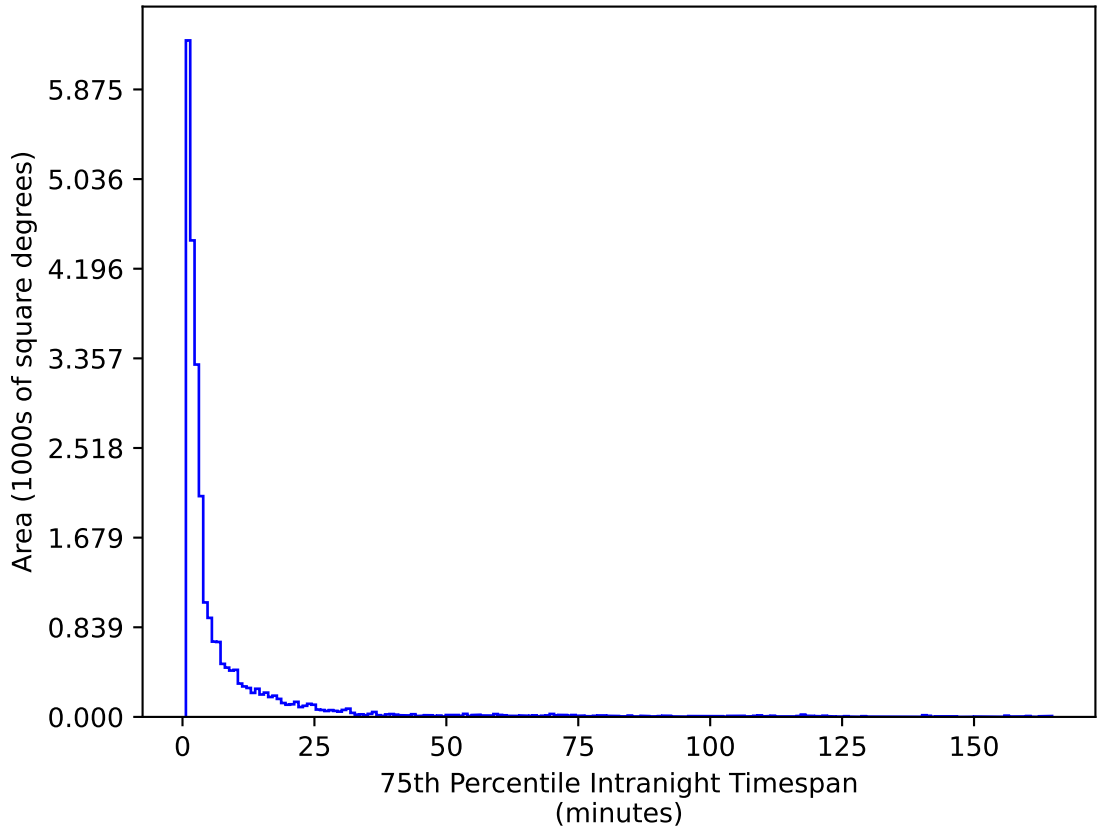
too_elab_r16_d3_ugrizy_v3.4_10yrs All sky g band: 75th Percentile Intranight Timespan
