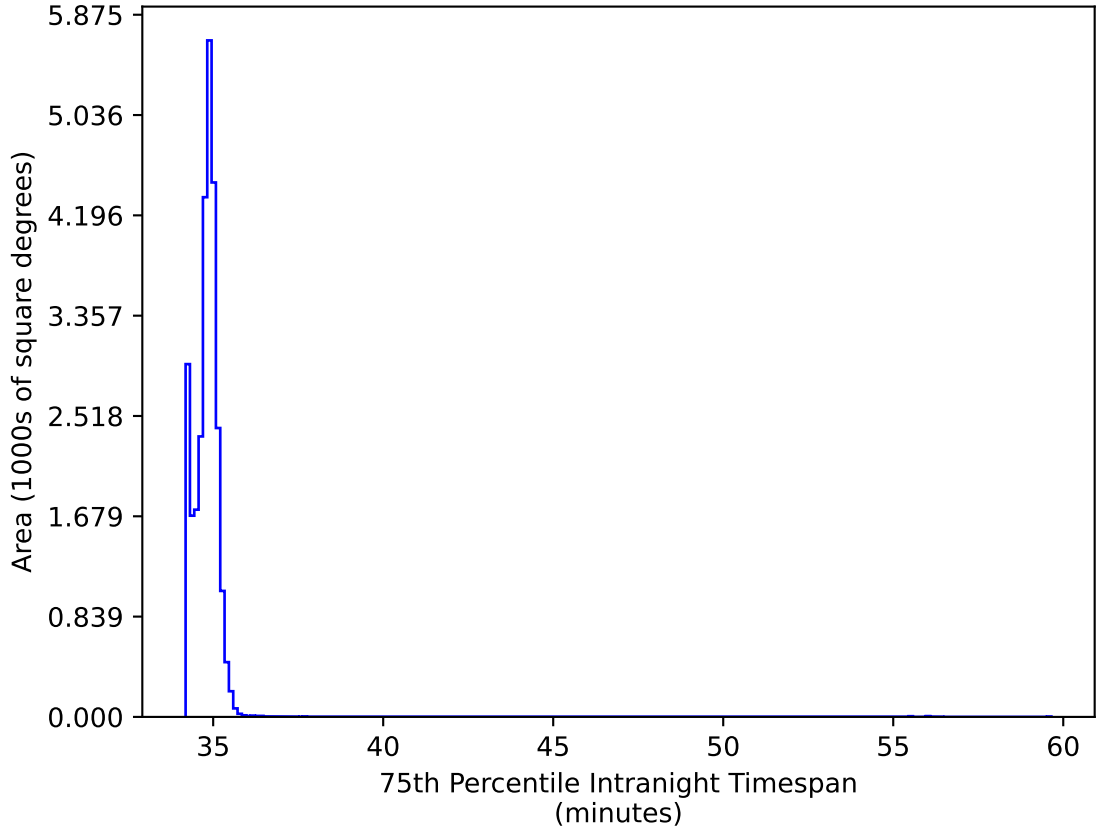
too_elab_r16_d3_ugrizy_v3.4_10yrs All sky all bands: 75th Percentile Intranight Timespan
