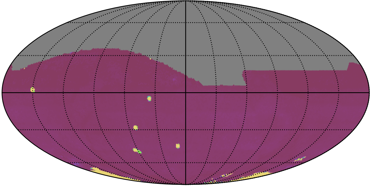
too_elab_r16_d3_ugrizy_v3.4_10yrs All sky: 75th Percentile Intranight Timespan
