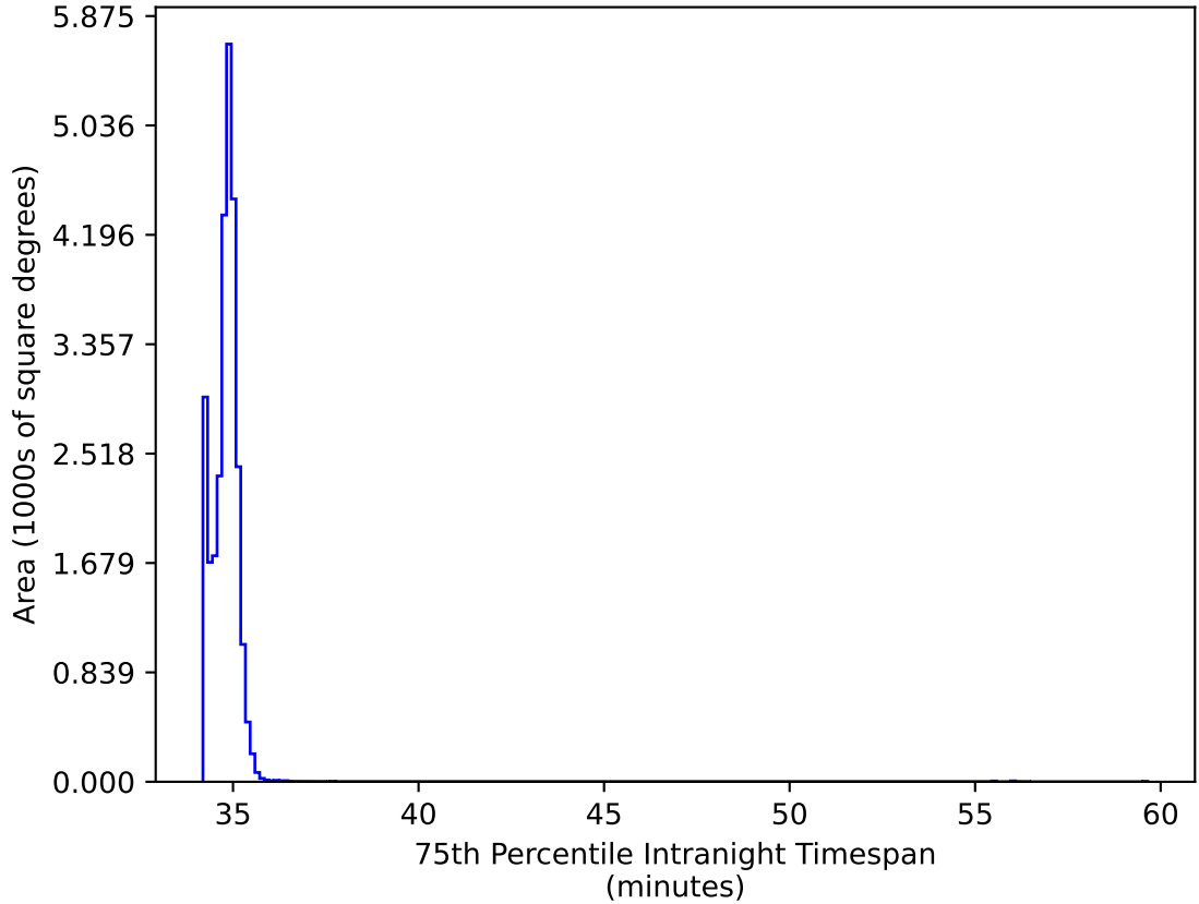
too_elab_r16_d3_ugrizy_v3.4_10yrs All sky: 75th Percentile Intranight Timespan
